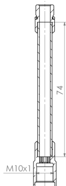
Page 4 L2 = 250 mm (Cu-Tube = 224 mm) weight = 60 g
